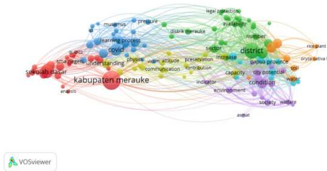
Gambar 1. Network Visualization
