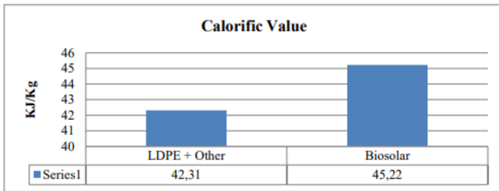
Figure 4. LDPE Calorific Value: Other and Biodiesel
