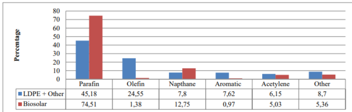
Figure 6. PONA Charts of Pyrolysis Oil and Biodiesel
