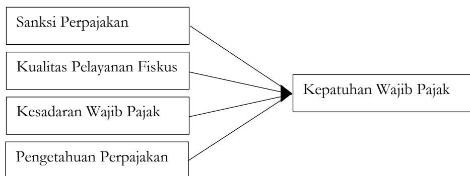
Gambar 2. Model penelitian
