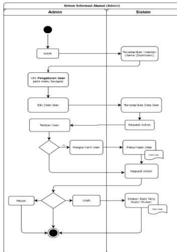
Gambar 4. 6 Activity Diagram Pengaturan User
