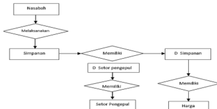
Gambar 3. Tampilan Flowchart
