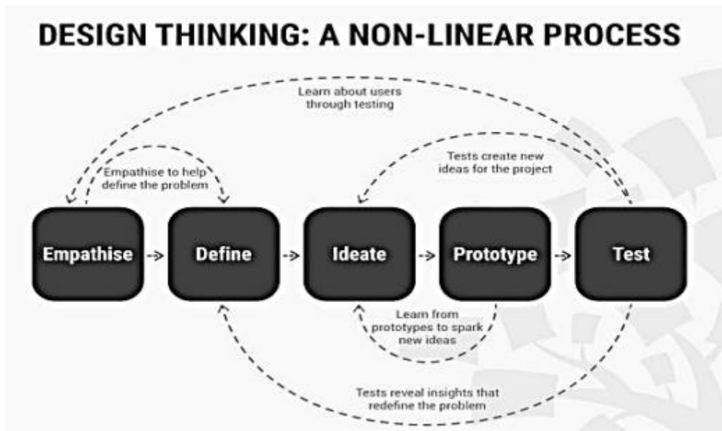
Gambar 2. Thinking Method
