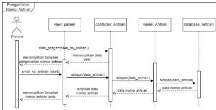
Gambar 4. Sequence Diagram
