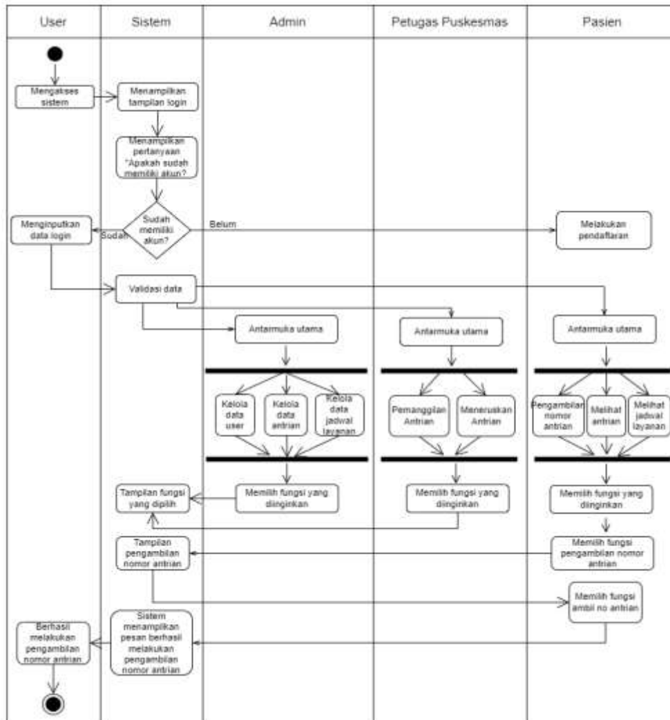
Gambar 3. Activity Diagram
