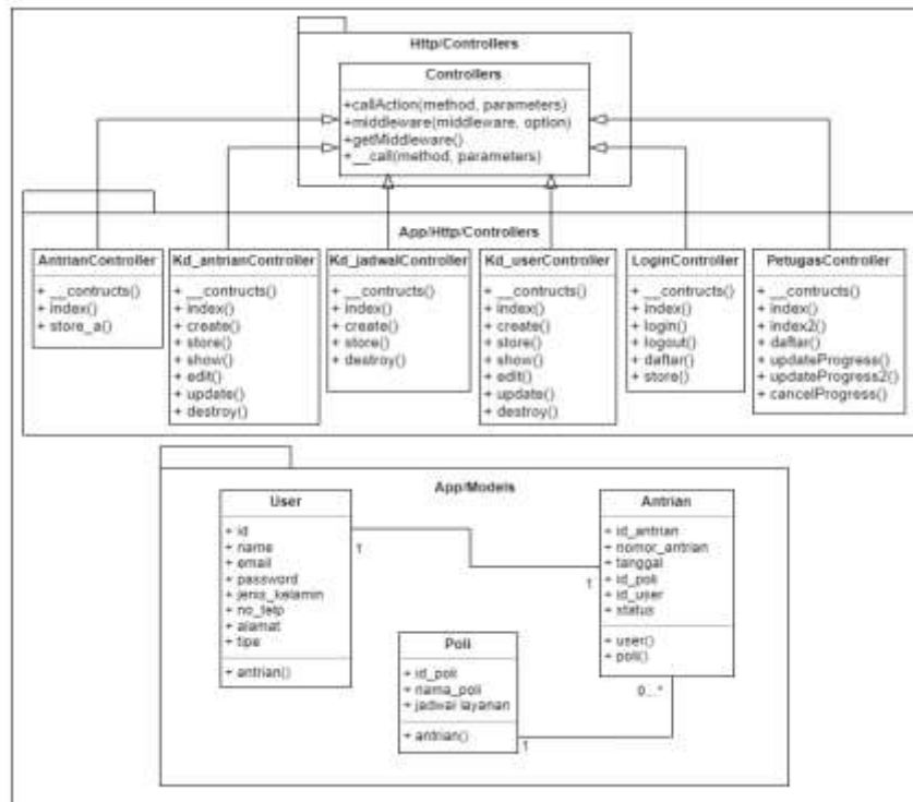
Gambar 5. Class Diagram
