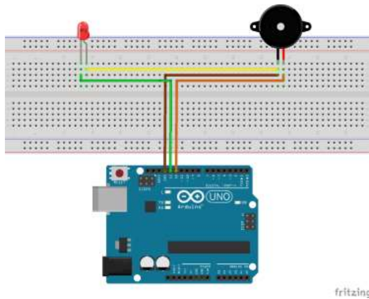
Gambar 4.5 schematic project
