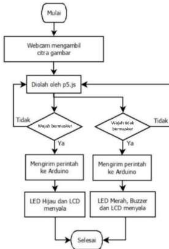
Gambar 3.1.1 Flowchart
