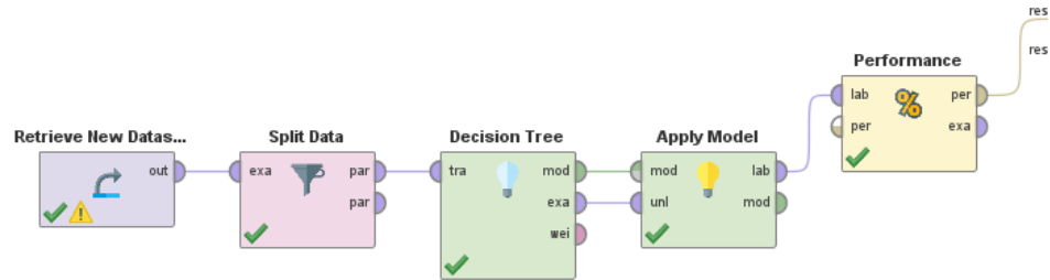
Gambar 4. 4 Proses Decision Tree C4.5 dan Split Validation
