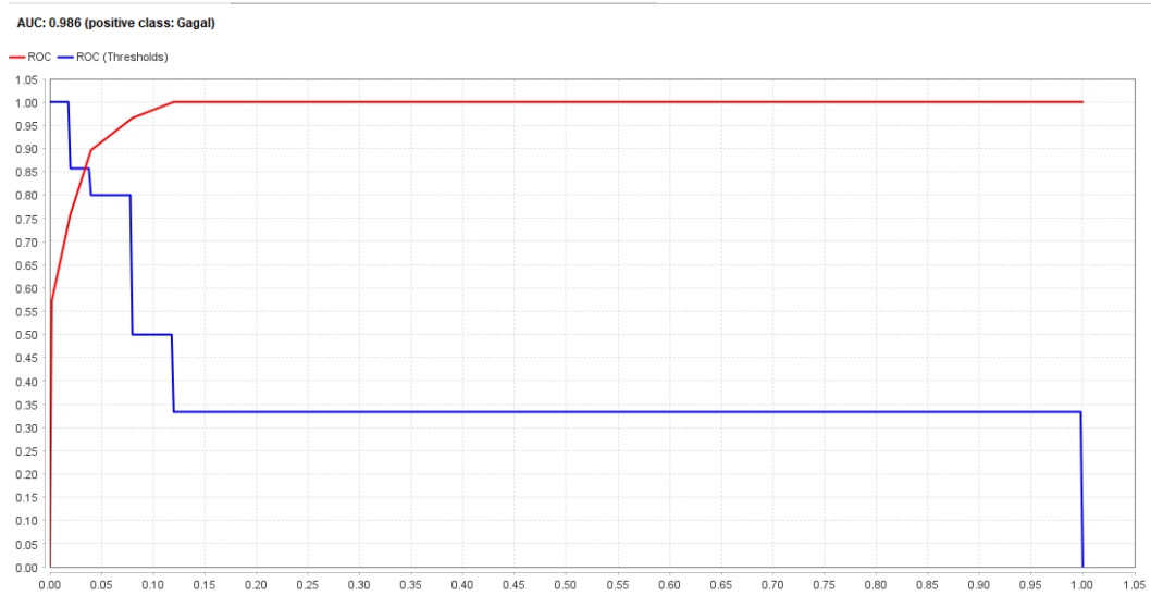
Gambar 4.8 Nilai AUC Algoritma Decision Tree
