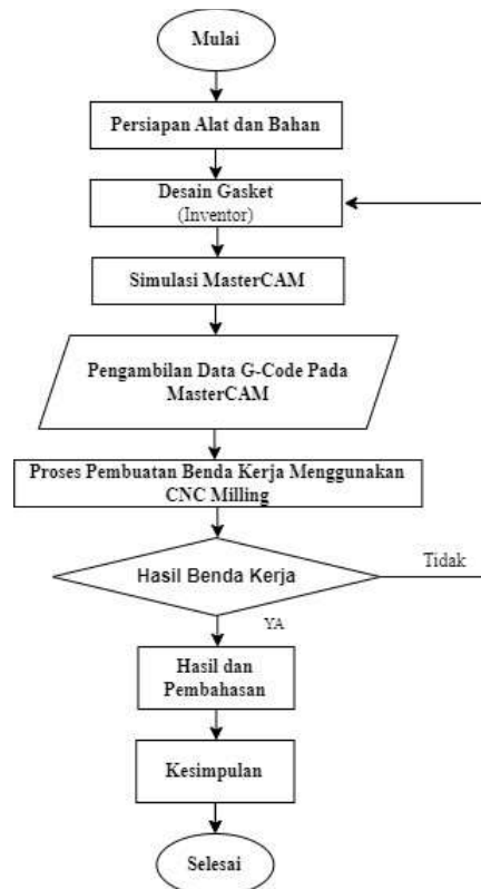
Gambar 1. Diagram Alir
